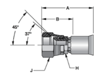
10691N Female SAE (JIC) 37° Swivel
